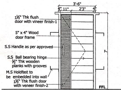
ELEVATION - MD (3'-6" x 7'-0")
